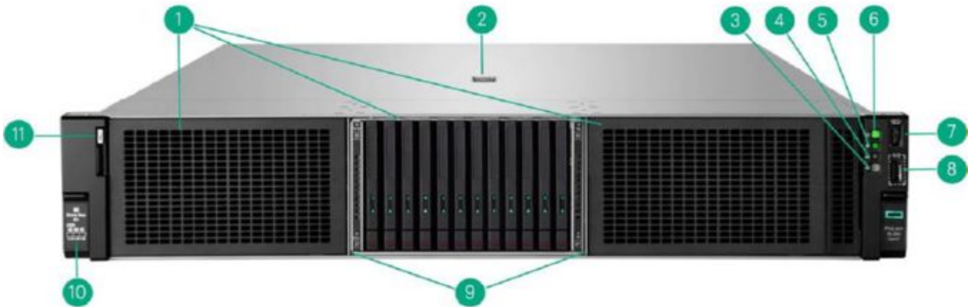
Front View -12EDSFF chassis shown
